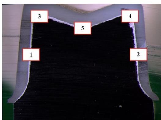
Figure 3. Five areas selected for the measurements using a Stereoscopic Microscope at 1.6\times magnification.
